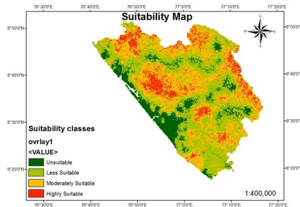
Figure 11: Landfill suitability map
